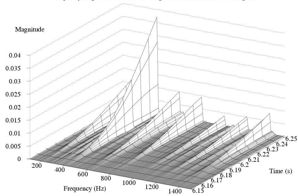
Spec3dw plot 18-09-2007 12:18:51, file: a20070912-saksalainen.raw, sampling rate: 44100Hz, FFT points: 8192, window length: 8192, type: hanning, increment: 400, frequency range: 100-1500Hz, HF weight: 1, comment: Saksalainen, g-kieli
