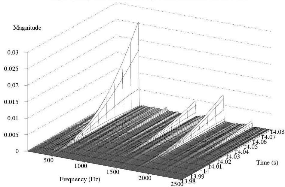
Spec3dw plot 18-09-2007 12:15:29, file: a20070912-saksalainen.raw, sampling rate: 44100Hz, FFT points: 8192, window length: 8192, type: hanning, increment: 400, frequency range: 100-2500Hz, HF weight: 1, comment: Saksalainen, a-kieli
