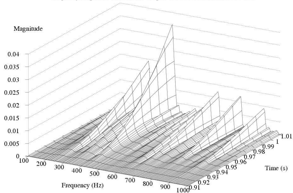
Spec3dw plot 18-09-2007 12:35:27, file: a20070912-saksalainen.raw, sampling rate: 44100Hz, FFT points: 8192, window length: 8192, type: hanning, increment: 400, frequency range: 100-1000Hz, HF weight: 1, comment: Saksalainen, c-kieli
