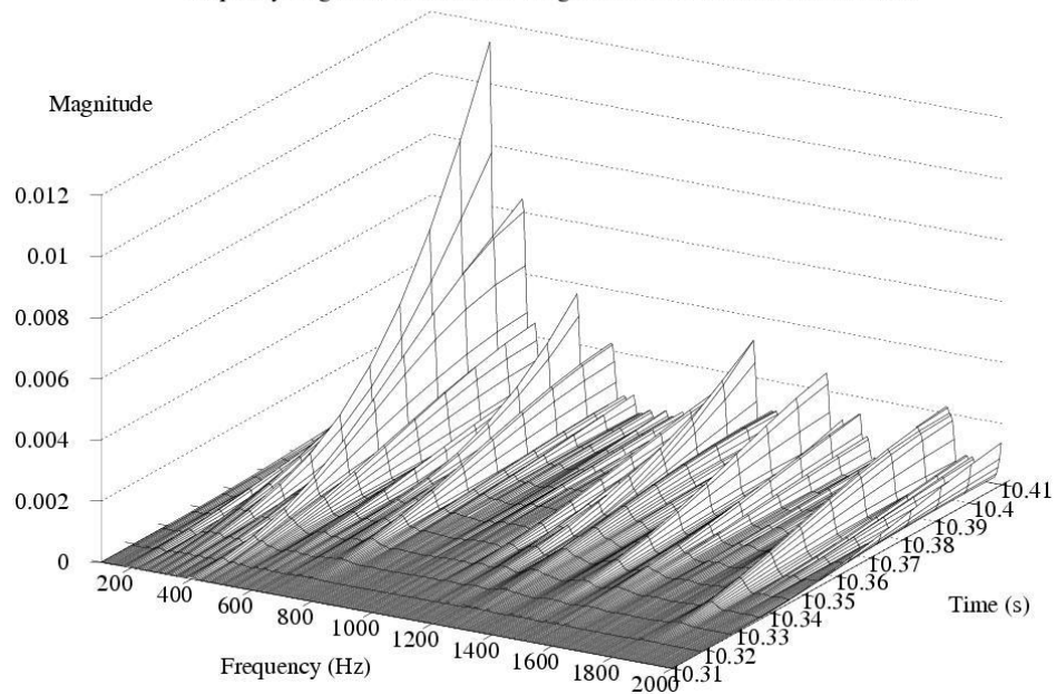
Spec3dw plot 18-09-2007 11:53:42, file: a20070912-saksalainen.raw, sampling rate: 44100Hz, FFT points: 8192, window length: 8192, type: hanning, increment: 400, frequency range: 100-2000Hz, HF weight: 1, comment: Saksalainen, d-kieli
